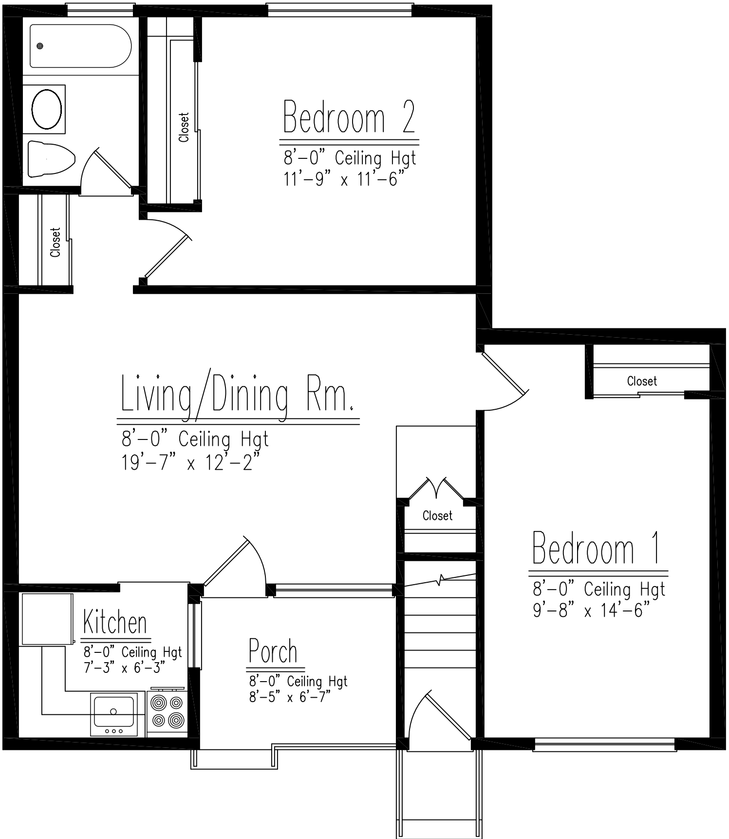
Type "E" - 2 Bedroom - 1st & 2nd Floor
